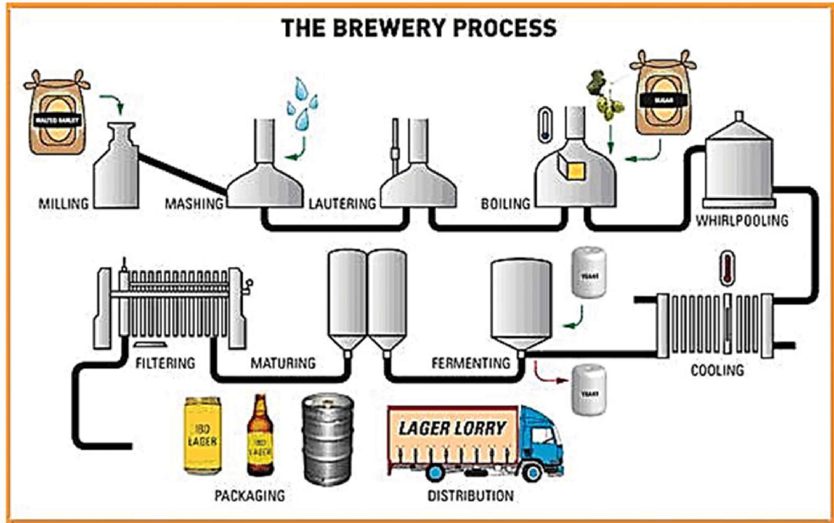
Figure 1. The Brewery Process
